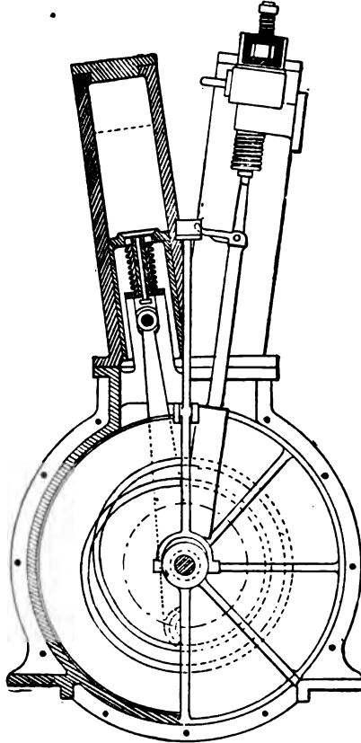
FIG. 363.—Part sectional view of the Daimler V-shaped Gasoline Engine, showing the air valve in the piston and eccentric cam grooves on the fly-wheel disc. The method of opening the exhaust valve is also indicated.
